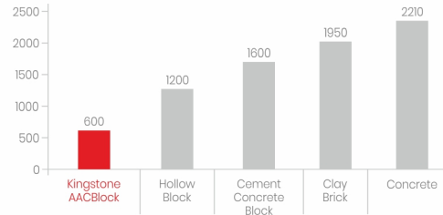
Density (Kg/M 3 ) of Various Materials
